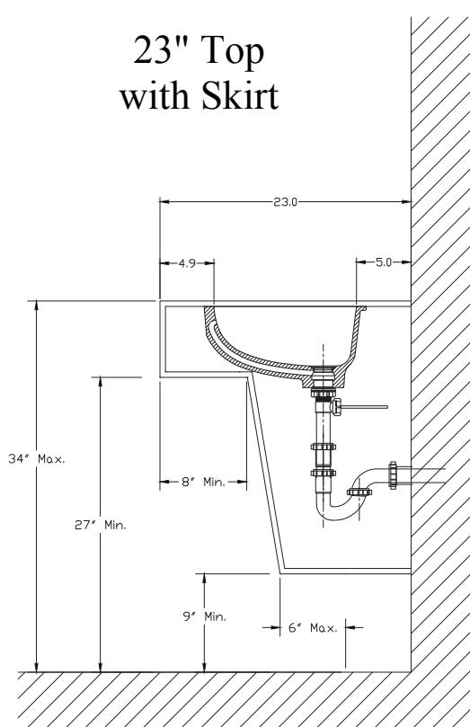
Figure E-3: DuPont™ Corian® 810P installation with Skirt
