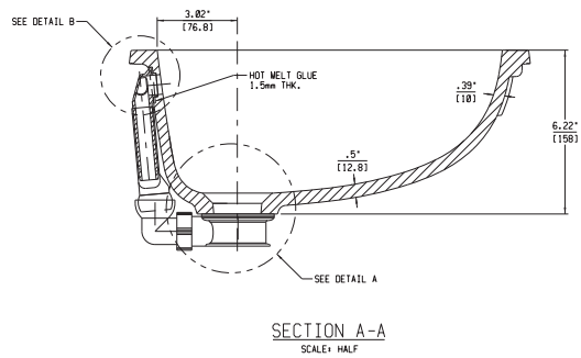
Figure D-4: DuPont™ Corian® 810 with Rear Overflow
