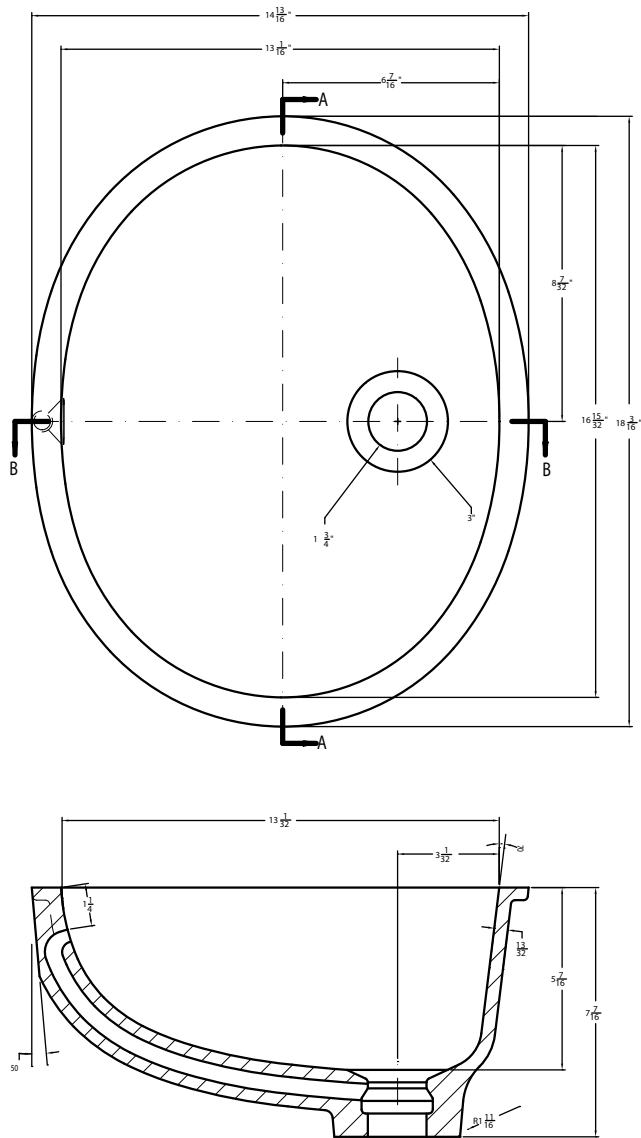
Figure E-1: DuPont™ Corian® 810P with Front or No Overflow
