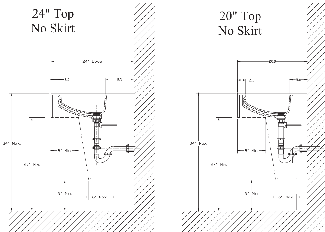
Figure N-3: DuPont™ Corian® 8254 installation without Skirt
