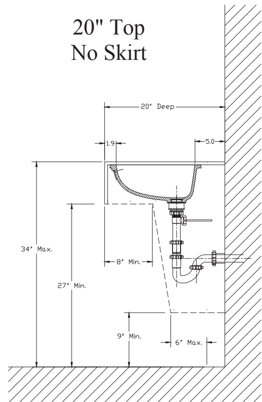
Figure D-6: DuPont™ Corian® 810 installation without Skirt
