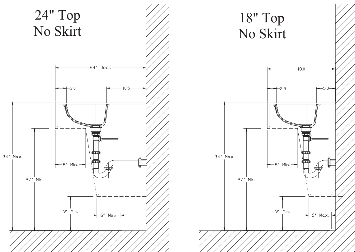
Figure H-5: DuPont™ Corian® 820 installation without Skirt
