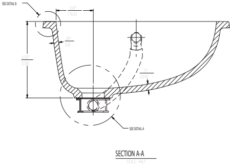
Figure D-3: DuPont™ Corian® 810 with Side Overflow
