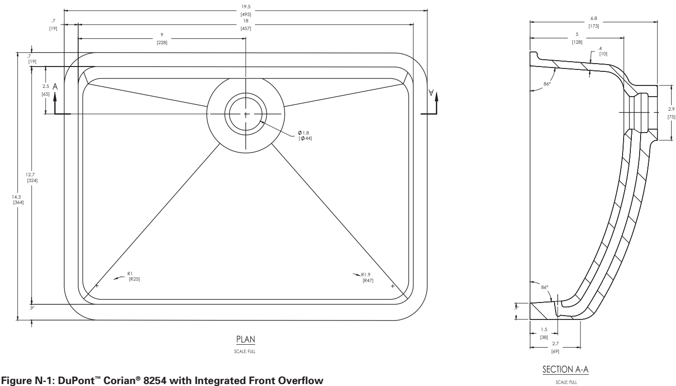
Figure N-1: DuPont™ Corian® 8254 with Integrated Front Overflow
